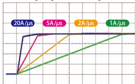
Ch4 load current 20A/div Horizontal 10us/div
