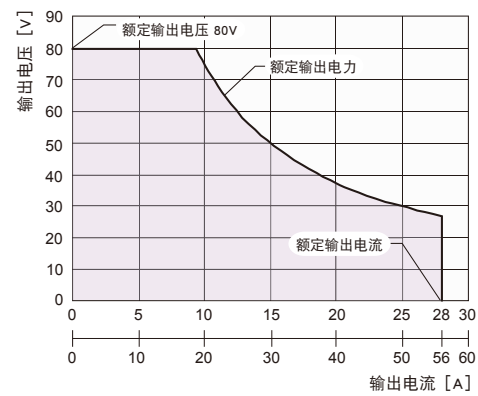
[ PWX750ML(MLF)/PWX1500ML ]
