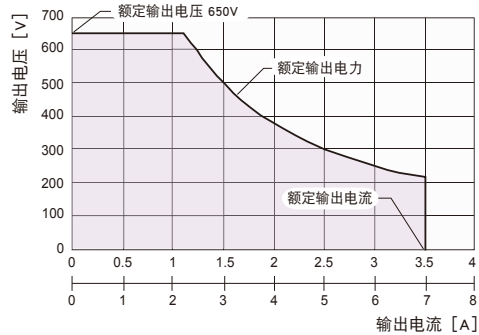
[ PWX750HF/PWX1500H ]
