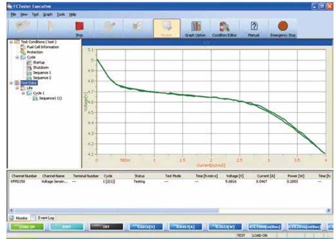
▲ I-V characteristics window
