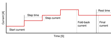
▲ I-V measurement
