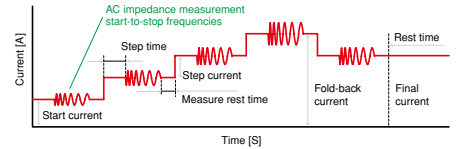
▲ I-V + Cole-Cole plot measurement
