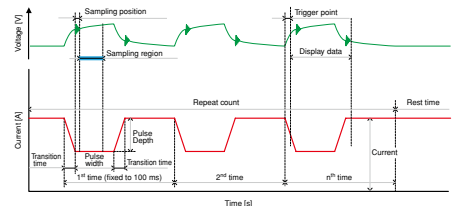
▲ Current interrupt measurement
